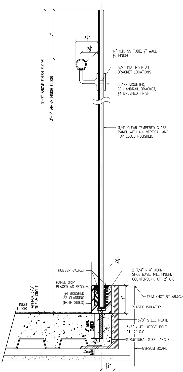
JOB # 764 LEVEL RAIL
