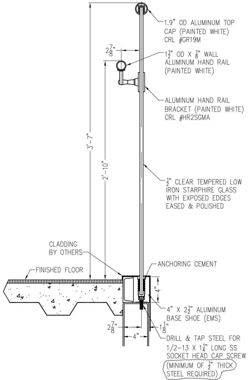
JOB # 919 STAIR RAIL
