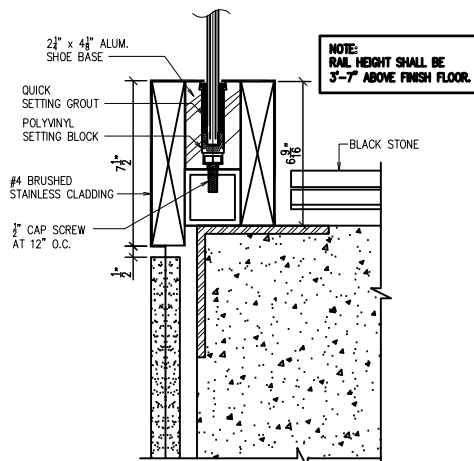
JOB # 656 LEVEL RAIL MOUNTING #4
