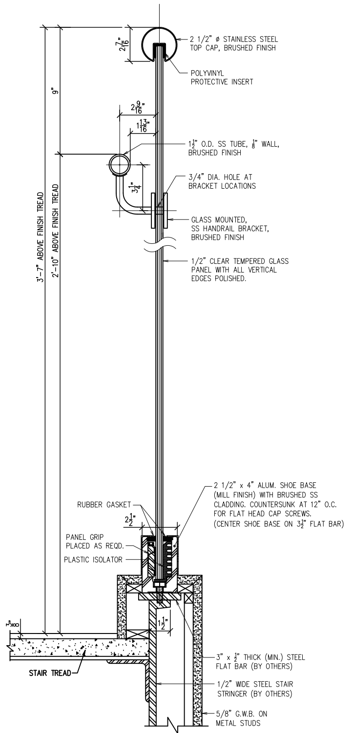
JOB # 758 STAIR RAIL
