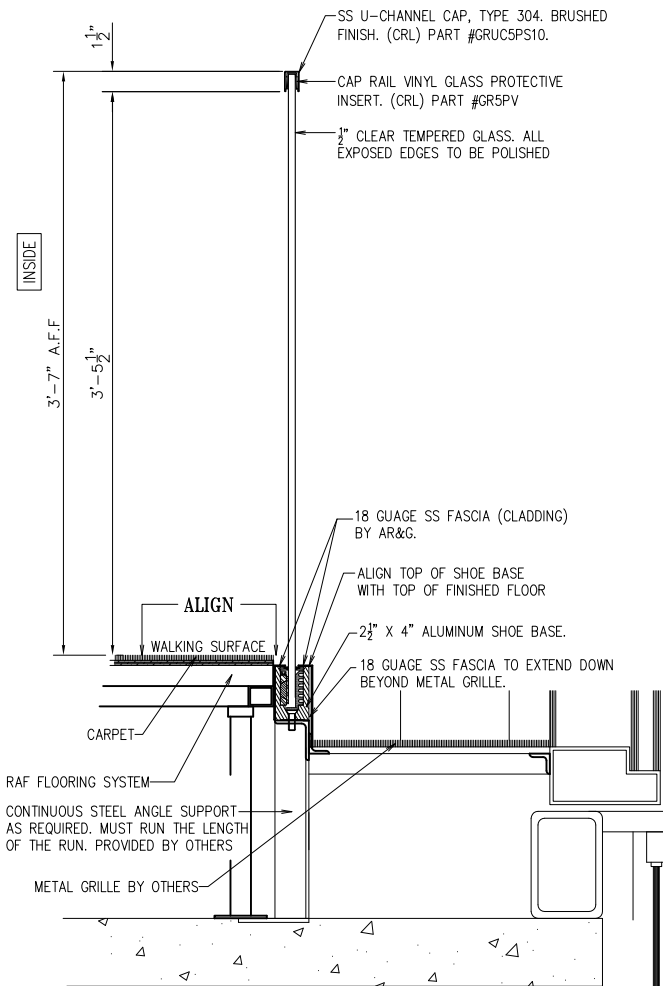
JOB # 772 LEVEL RAIL
