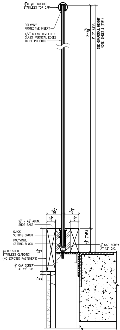
JOB # 656 LEVEL RAIL MOUNTING #1
