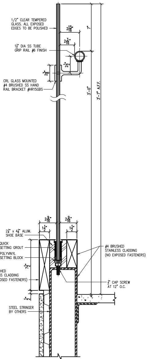
JOB # 656 STAIR RAIL MOUNTING #2
