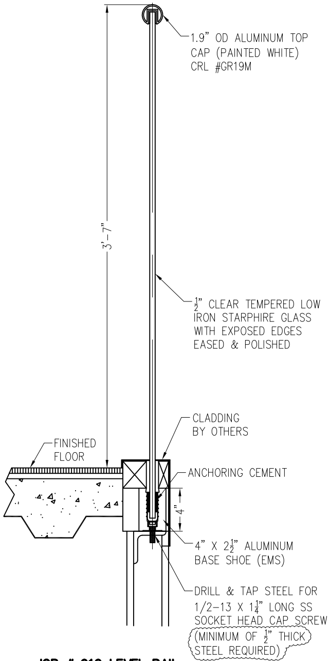
JOB # 919 LEVEL RAIL
