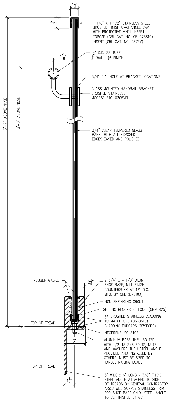
JOB # 775 STAIR RAIL
