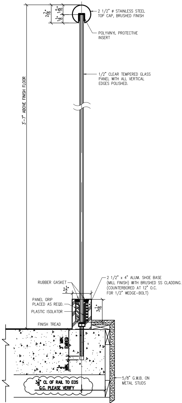
JOB # 758 LEVEL RAIL
