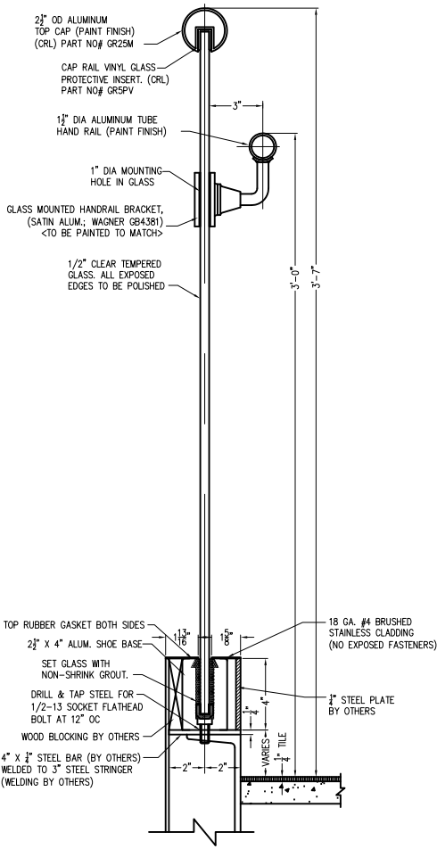
SECTION THRU - STAIR & LANDING RAIL 'GS'
