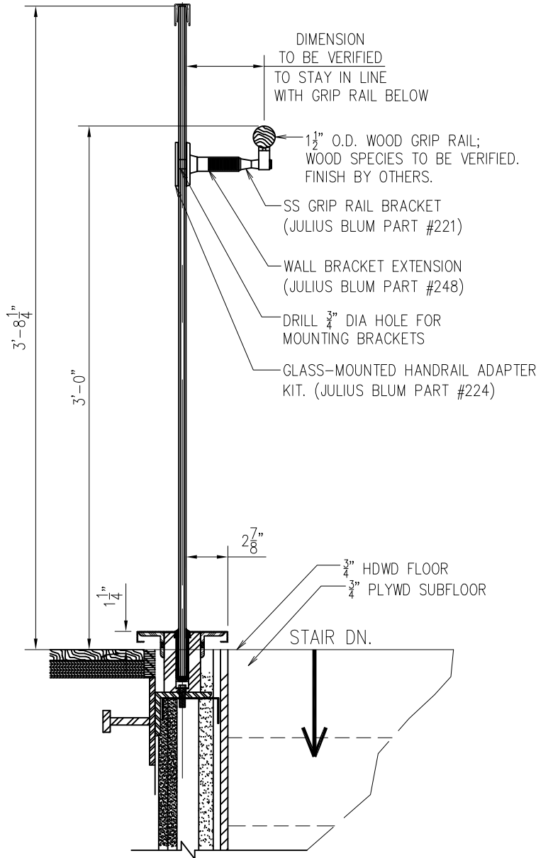
JOB # 718 STAIR RAIL
