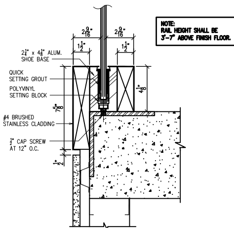
JOB # 656 LEVEL RAIL MOUNTING #3
