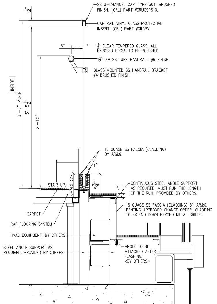
JOB # 772 STAIR RAIL
