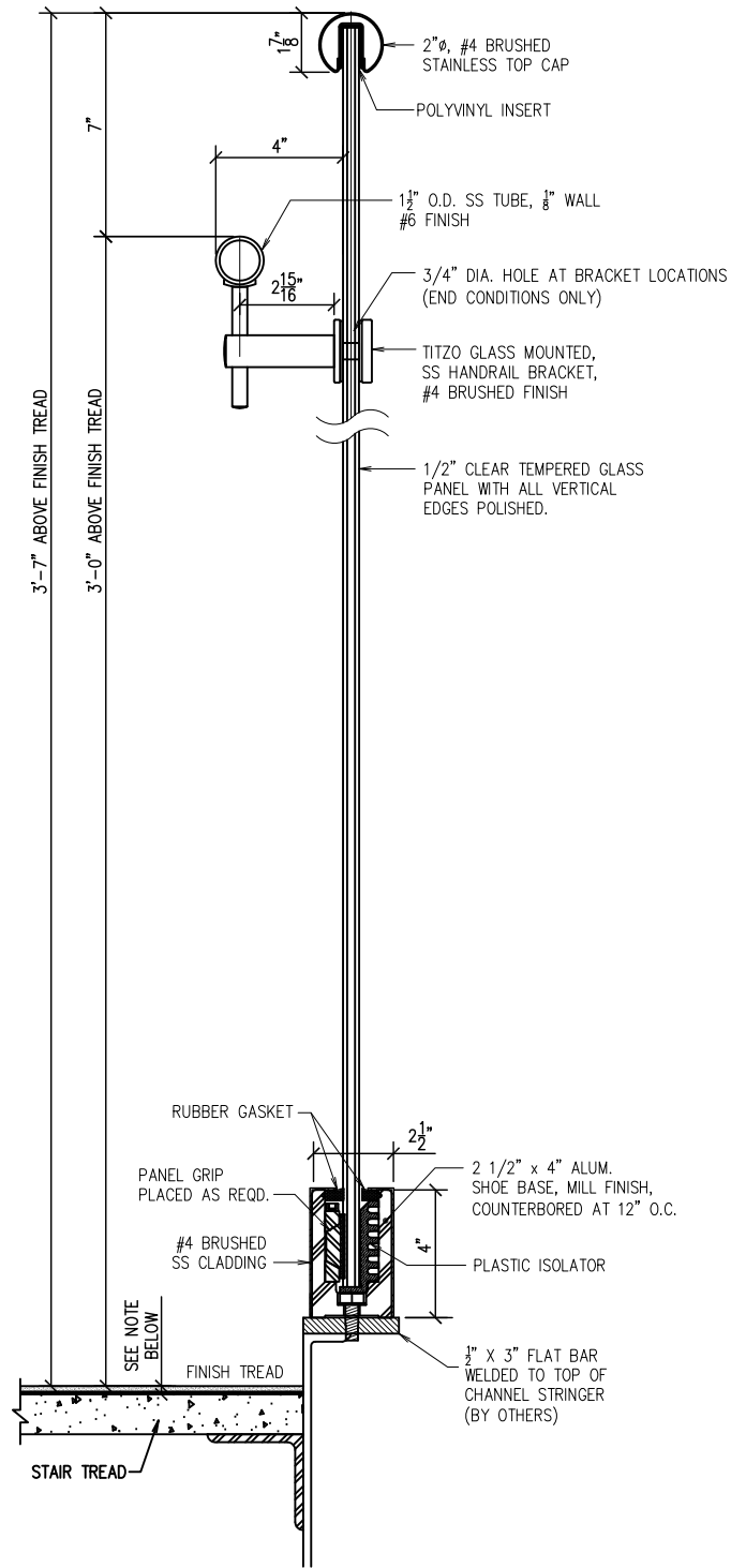
JOB # 751 STAIR RAIL
