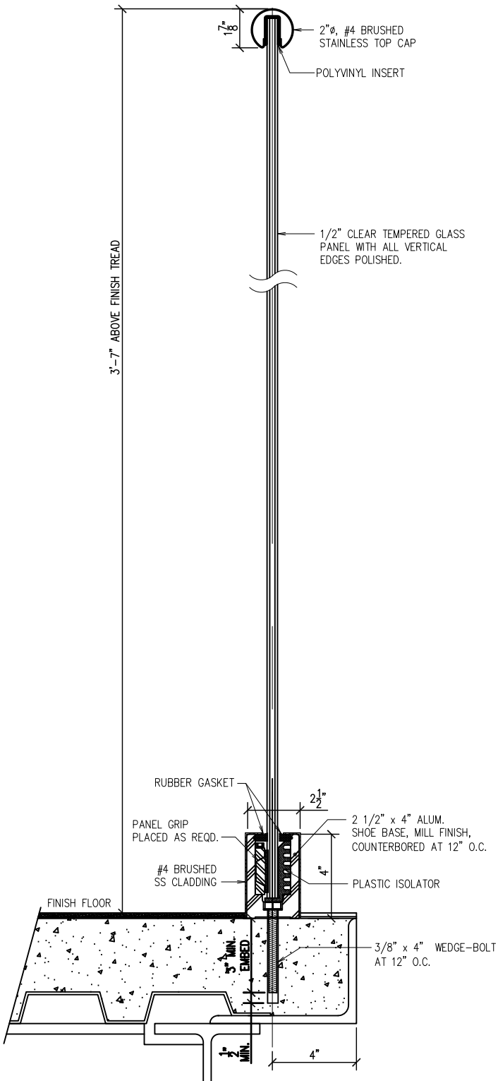
JOB # 751 LEVEL RAIL
