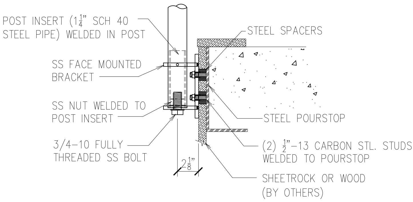
SIDE MOUNT ATTACHED TO POURSTOP OVER WOOD FASCIA OR SHEETROCK
