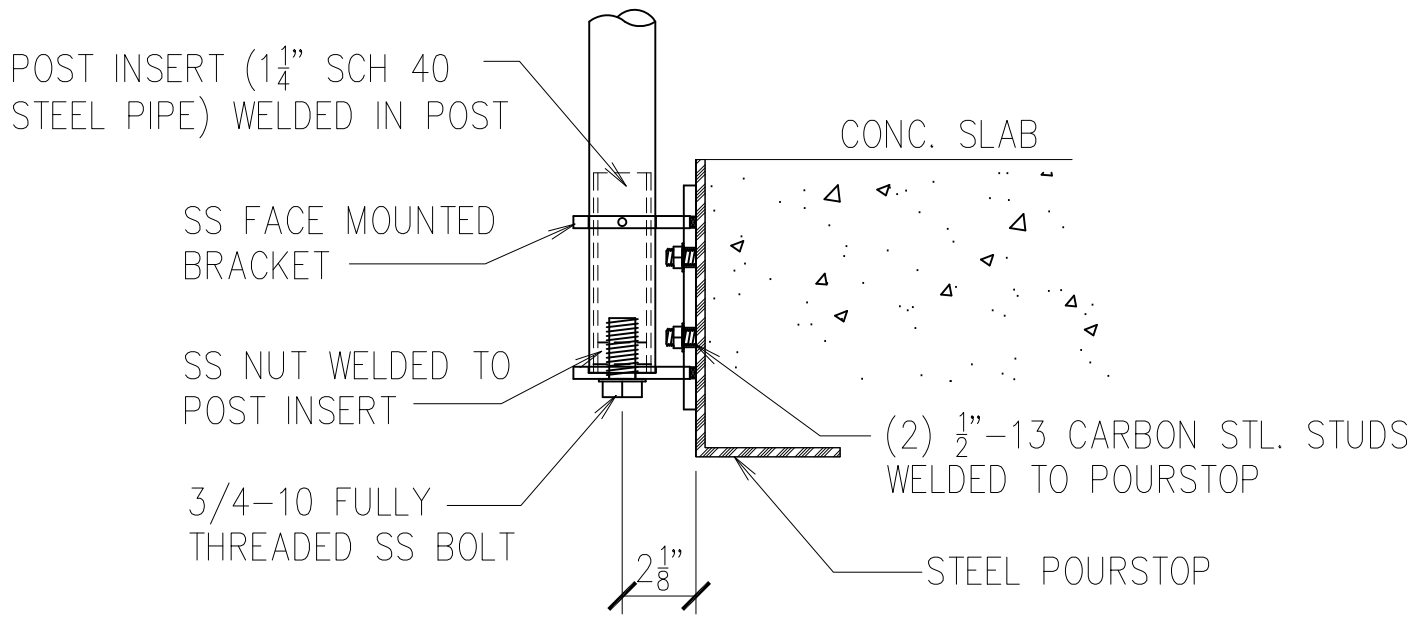
SIDE MOUNT ATTACHED TO POURSTOP
